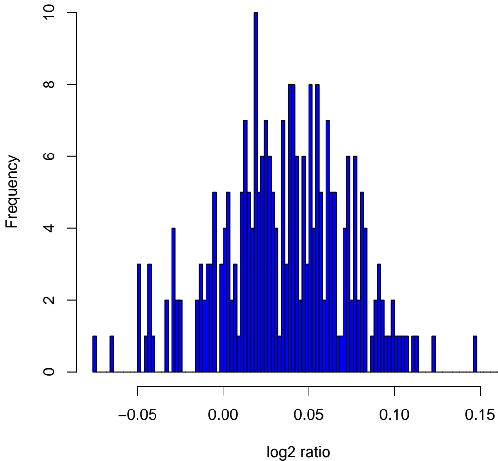
Histogram of log2ratios in 270 HapMap samples at clone Chr17tp-10D5
