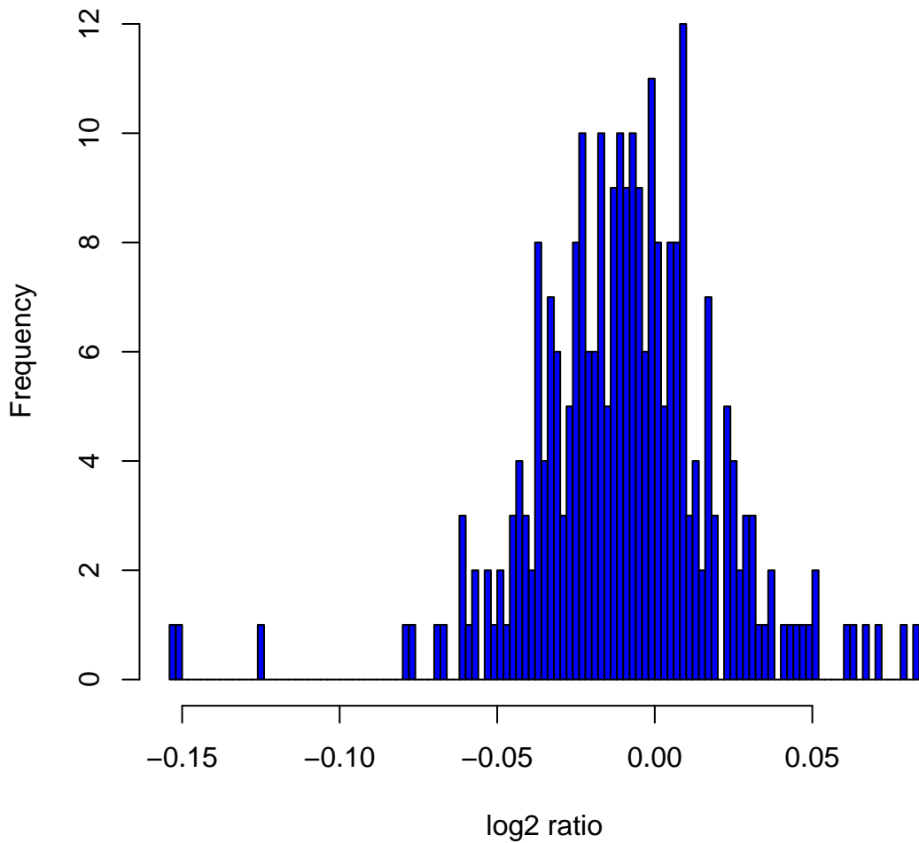
Histogram of log2ratios in 270 HapMap samples at clone Chr17tp-10E10
