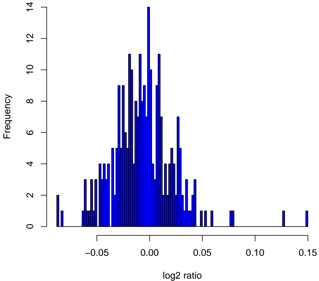
Histogram of log2ratios in 270 HapMap samples at clone Chr17tp-10E2
