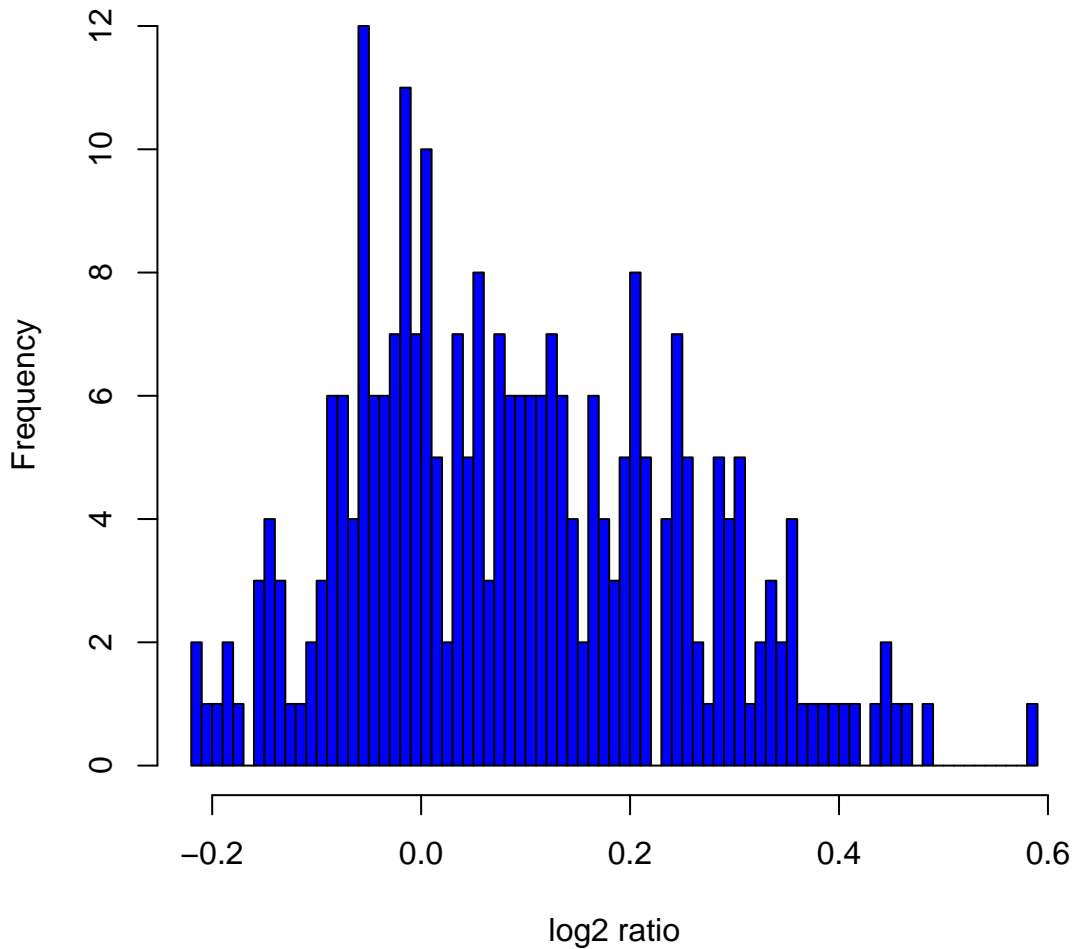
Histogram of \log_2 ratios in 270 HapMap samples at clone Chr17tp-10G2
