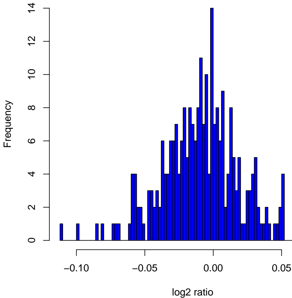
Histogram of log2ratios in 270 HapMap samples at clone Chr17tp-10H7
