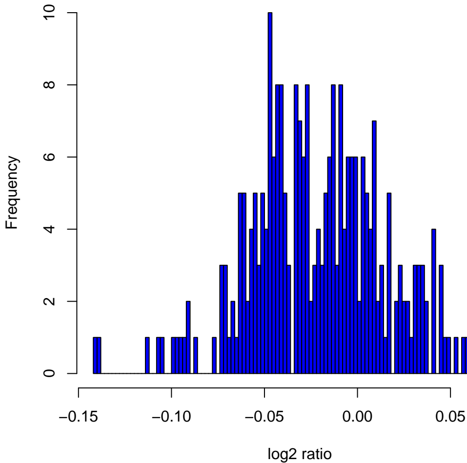
Histogram of log2ratios in 270 HapMap samples at clone Chr17tp-10H9
