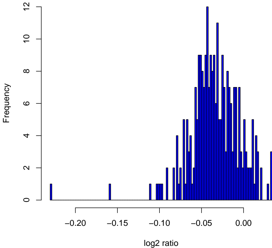
Histogram of log2ratios in 270 HapMap samples at clone Chr17tp-11A2
