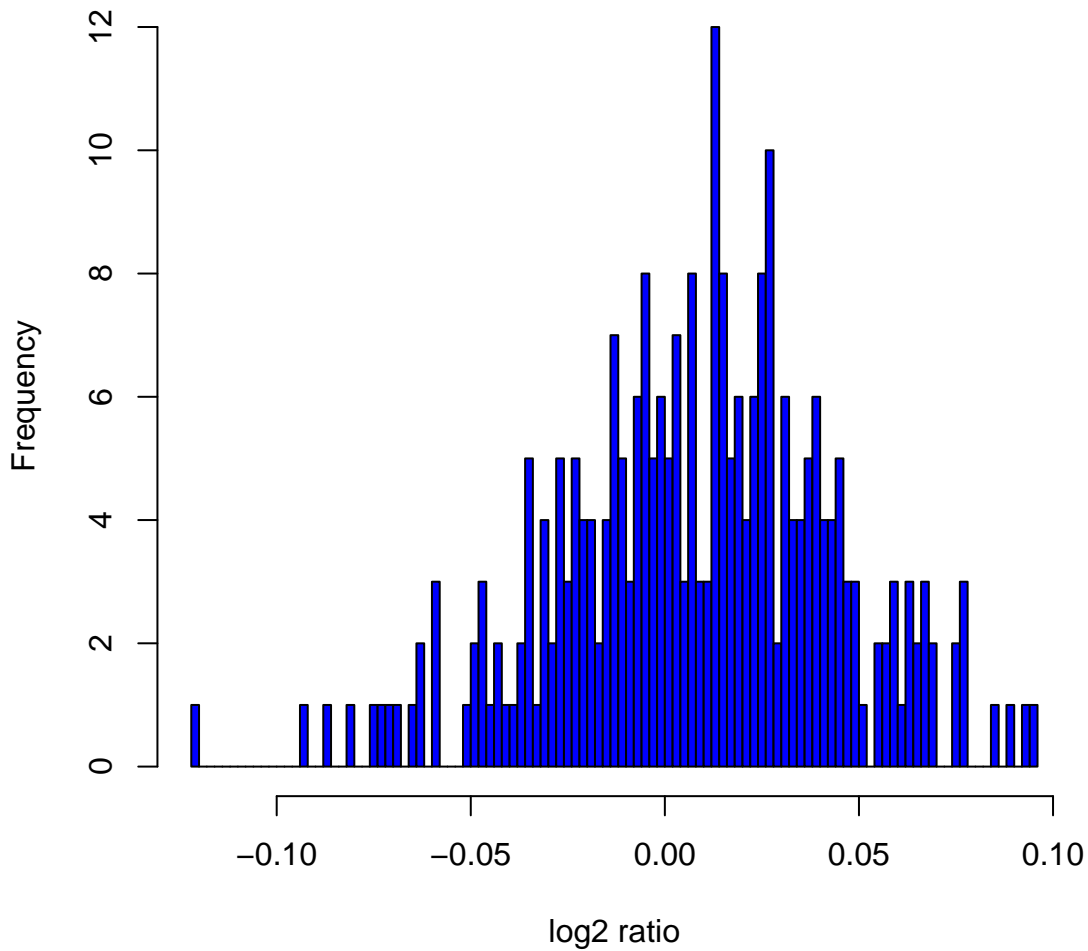
Histogram of log2ratios in 270 HapMap samples at clone Chr17tp-11B12
