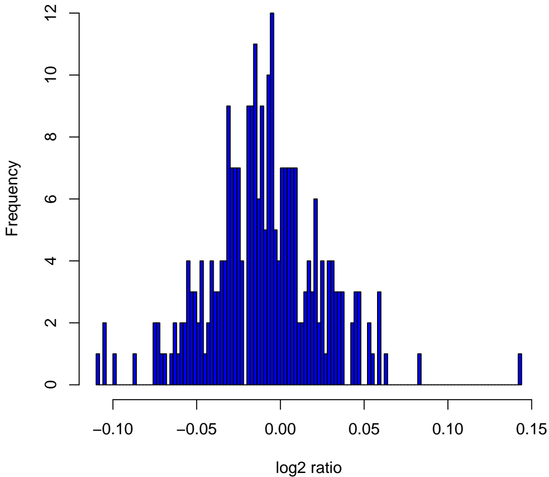
Histogram of log2ratios in 270 HapMap samples at clone Chr17tp-11C2
