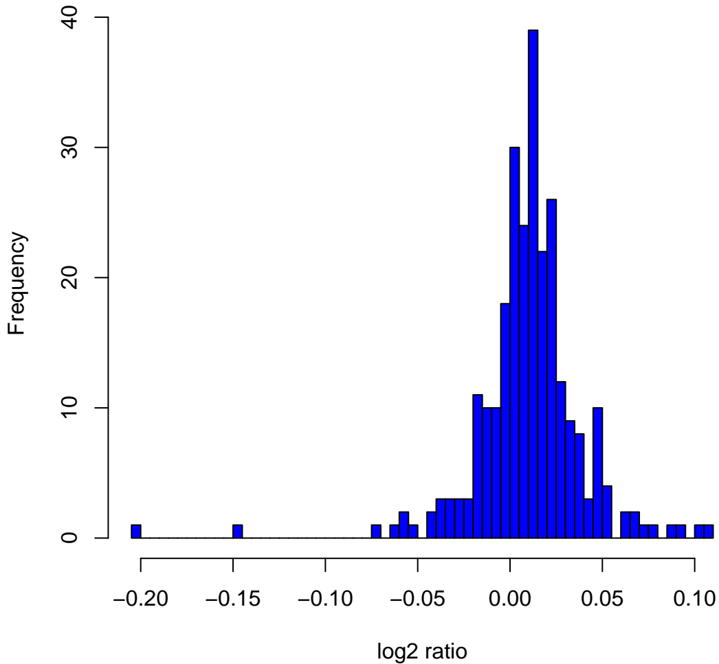
Histogram of log2ratios in 270 HapMap samples at clone Chr17tp-11C9
