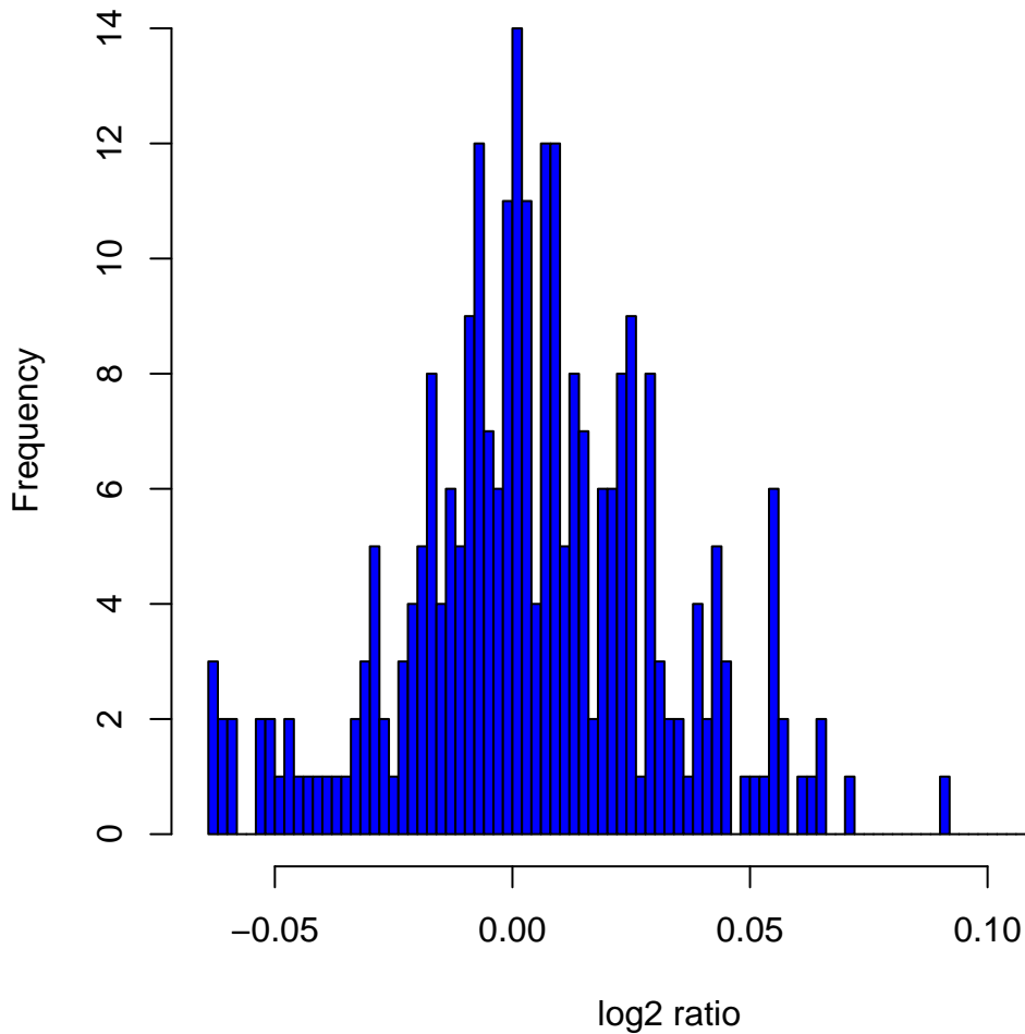
Histogram of log2ratios in 270 HapMap samples at clone Chr17tp-12B8
