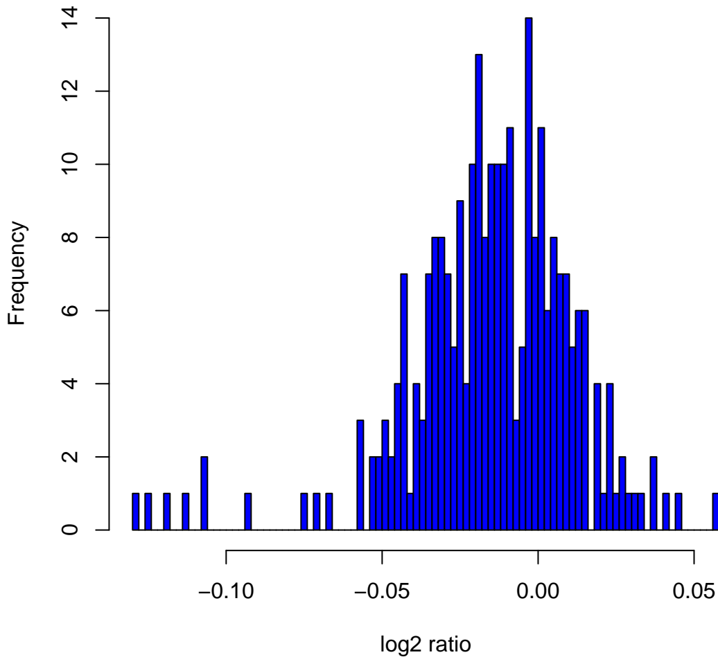
Histogram of log2ratios in 270 HapMap samples at clone Chr17tp-12C8
