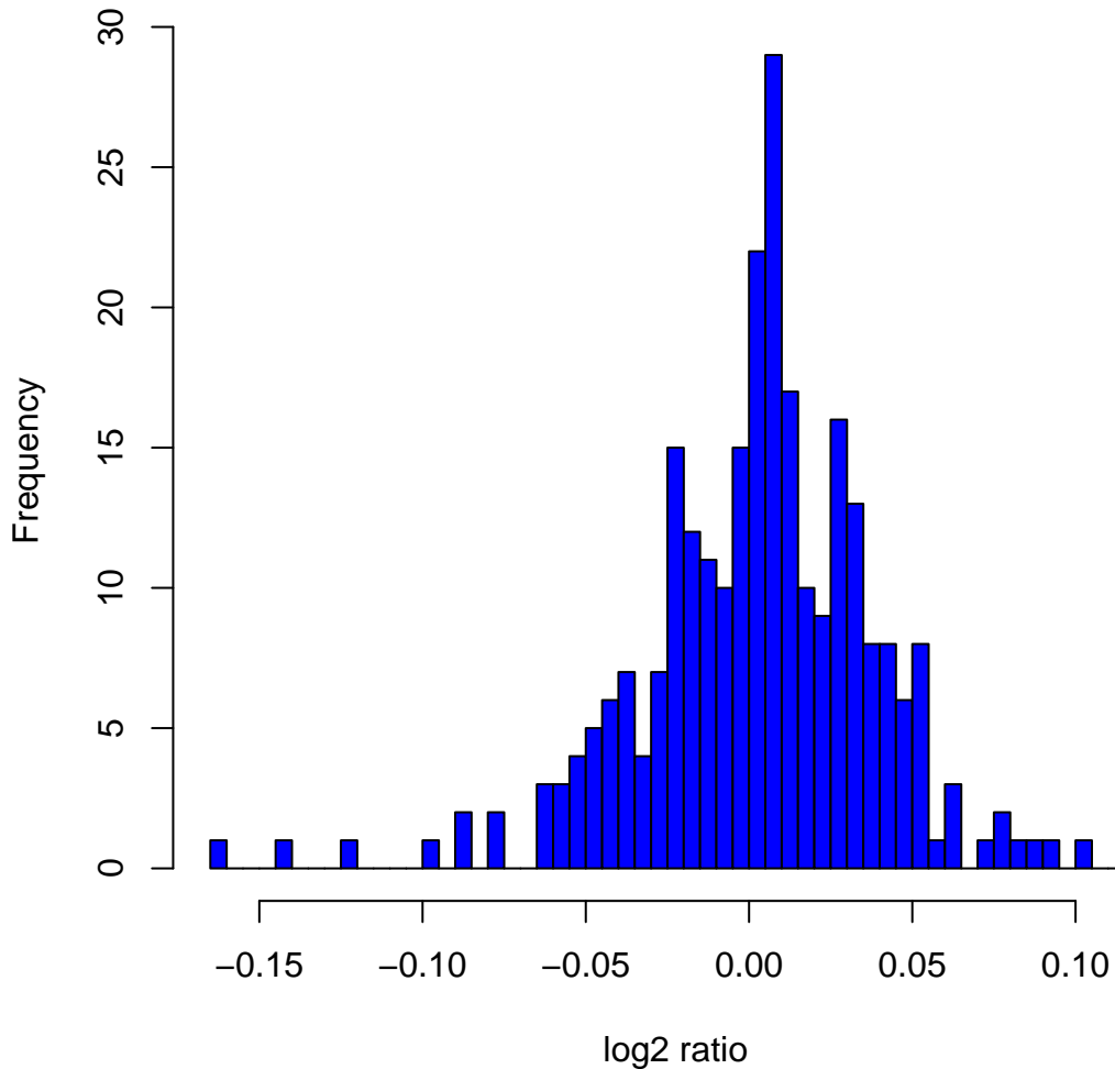
Histogram of log2ratios in 270 HapMap samples at clone Chr17tp-12E5
