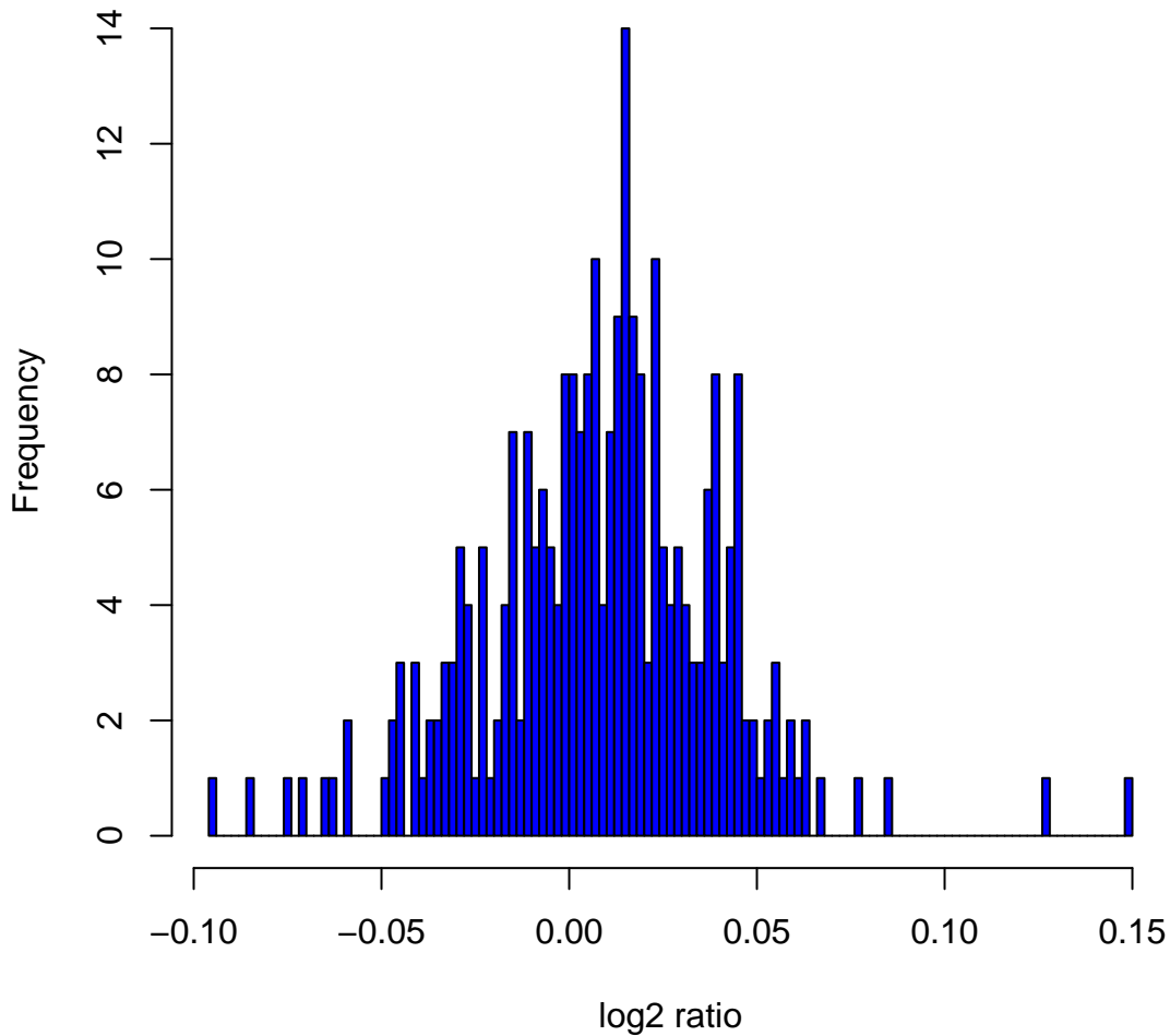
Histogram of log2ratios in 270 HapMap samples at clone Chr17tp-13A3
