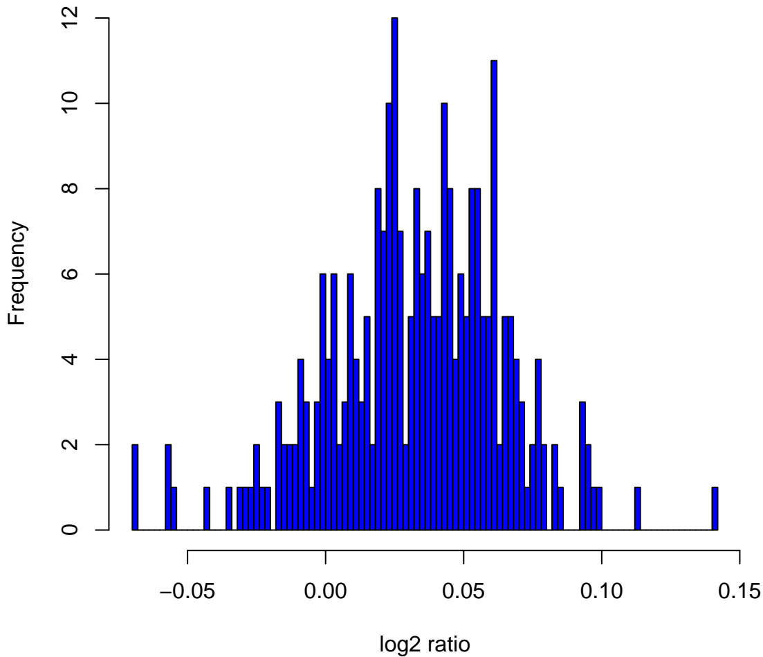
Histogram of log2ratios in 270 HapMap samples at clone Chr17tp-13A6
