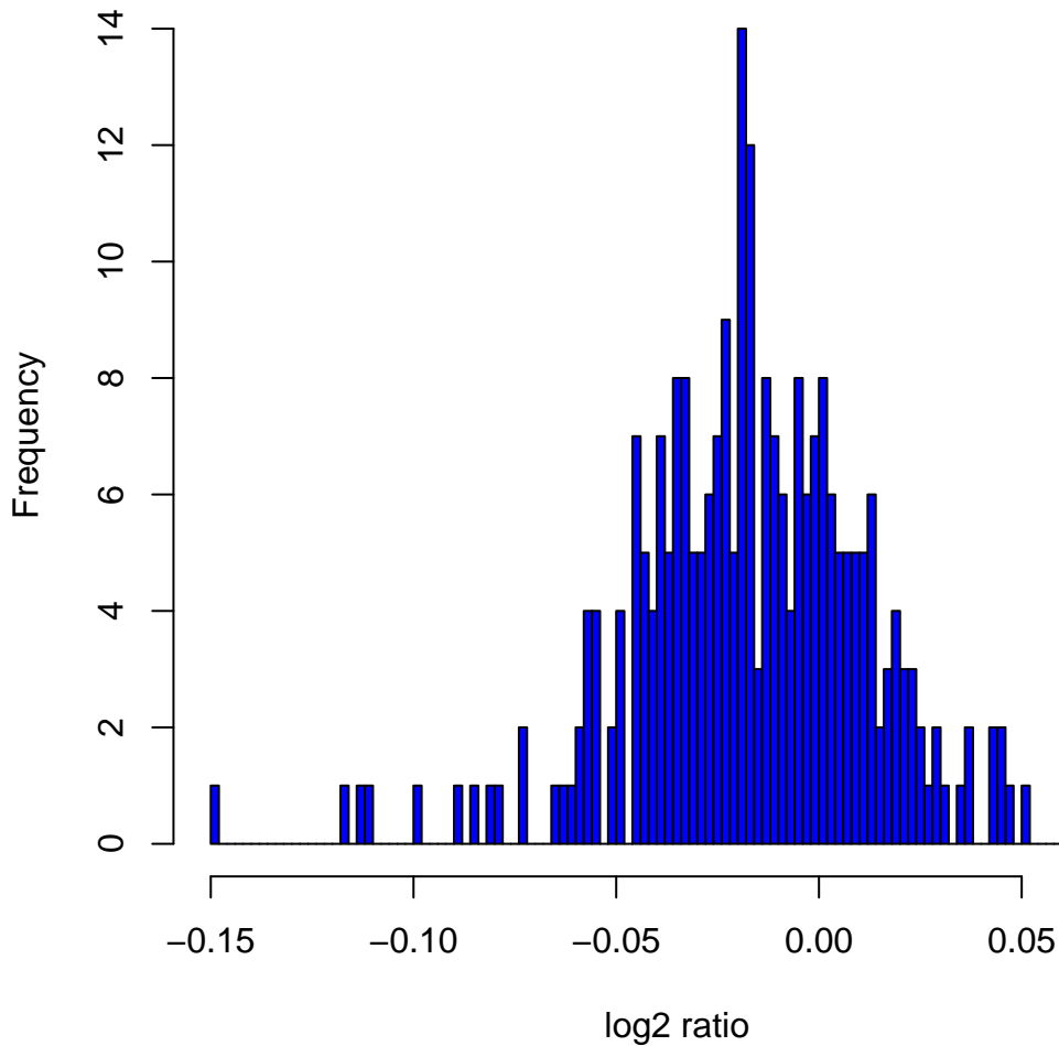
Histogram of log 2 ratios in 270 HapMap samples at clone Chr17tp-1F1
