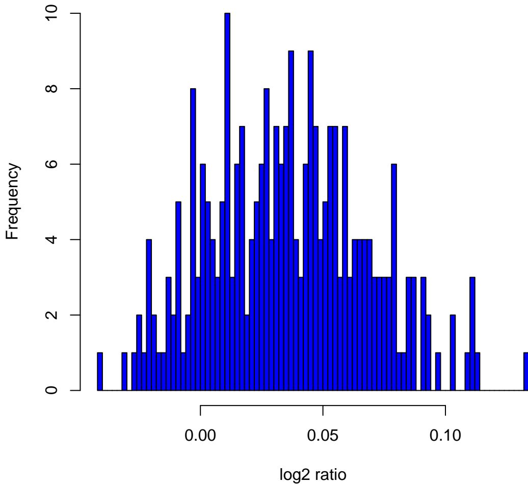
Histogram of log2ratios in 270 HapMap samples at clone Chr17tp-1F11
