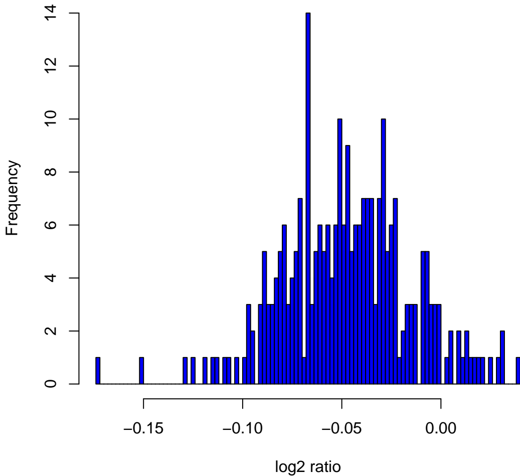
Histogram of log2ratios in 270 HapMap samples at clone Chr17tp-2B3
