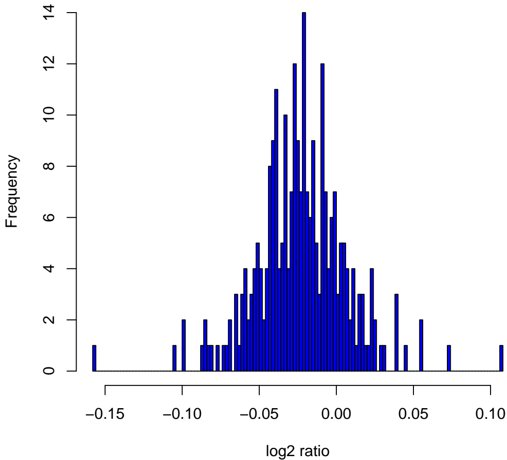
Histogram of log 2 ratios in 270 HapMap samples at clone Chr17tp-2D7
