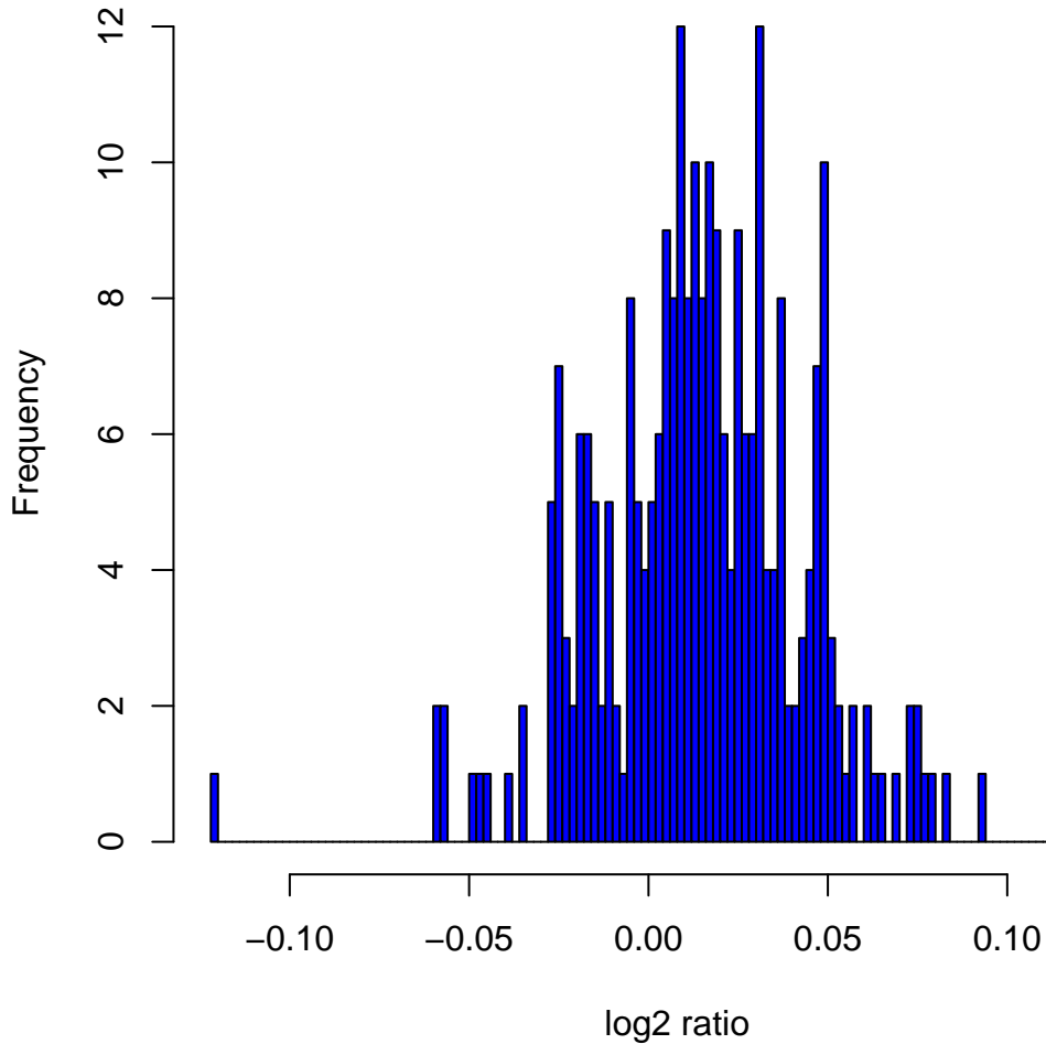
Histogram of log2ratios in 270 HapMap samples at clone Chr17tp-2E11
