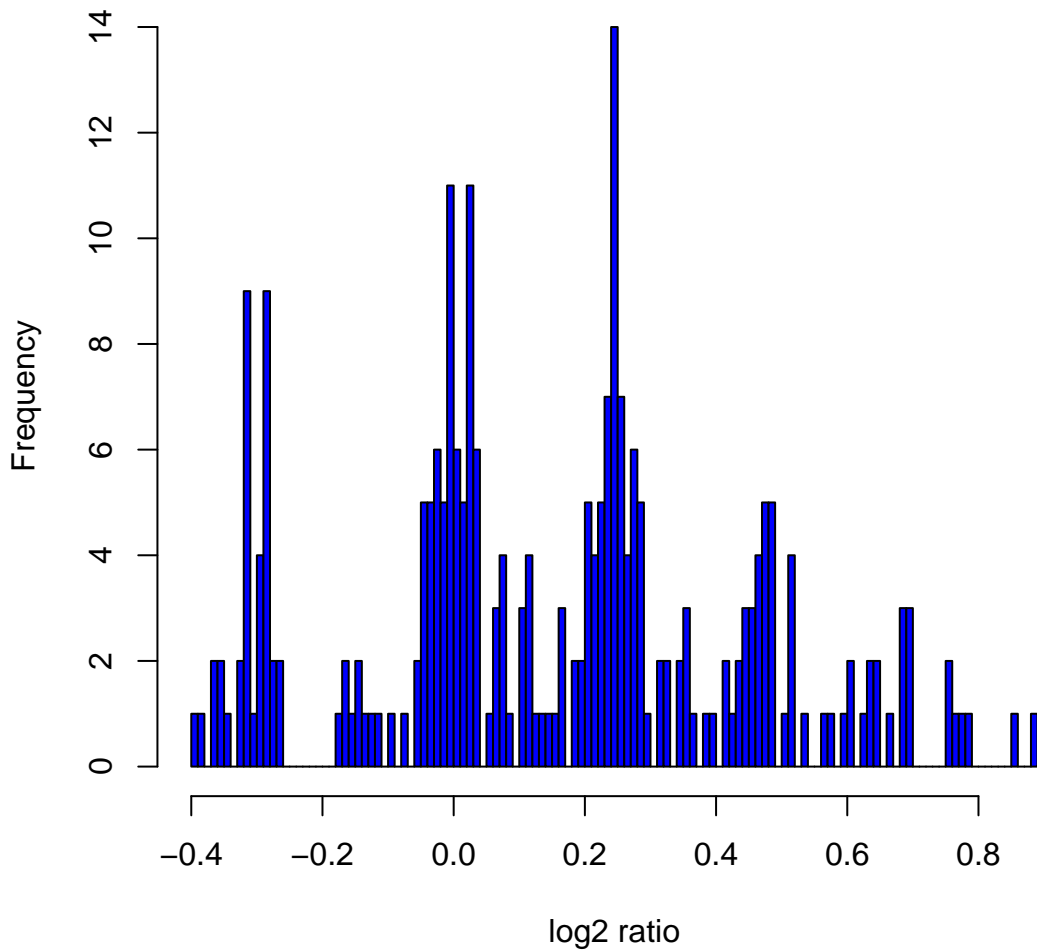
Histogram of log2ratios in 270 HapMap samples at clone Chr17tp-2F6
