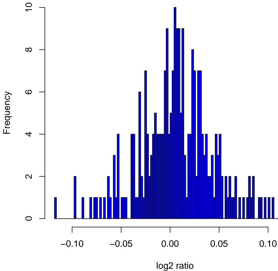
Histogram of \log_2 ratios in 270 HapMap samples at clone Chr17tp-3D4
