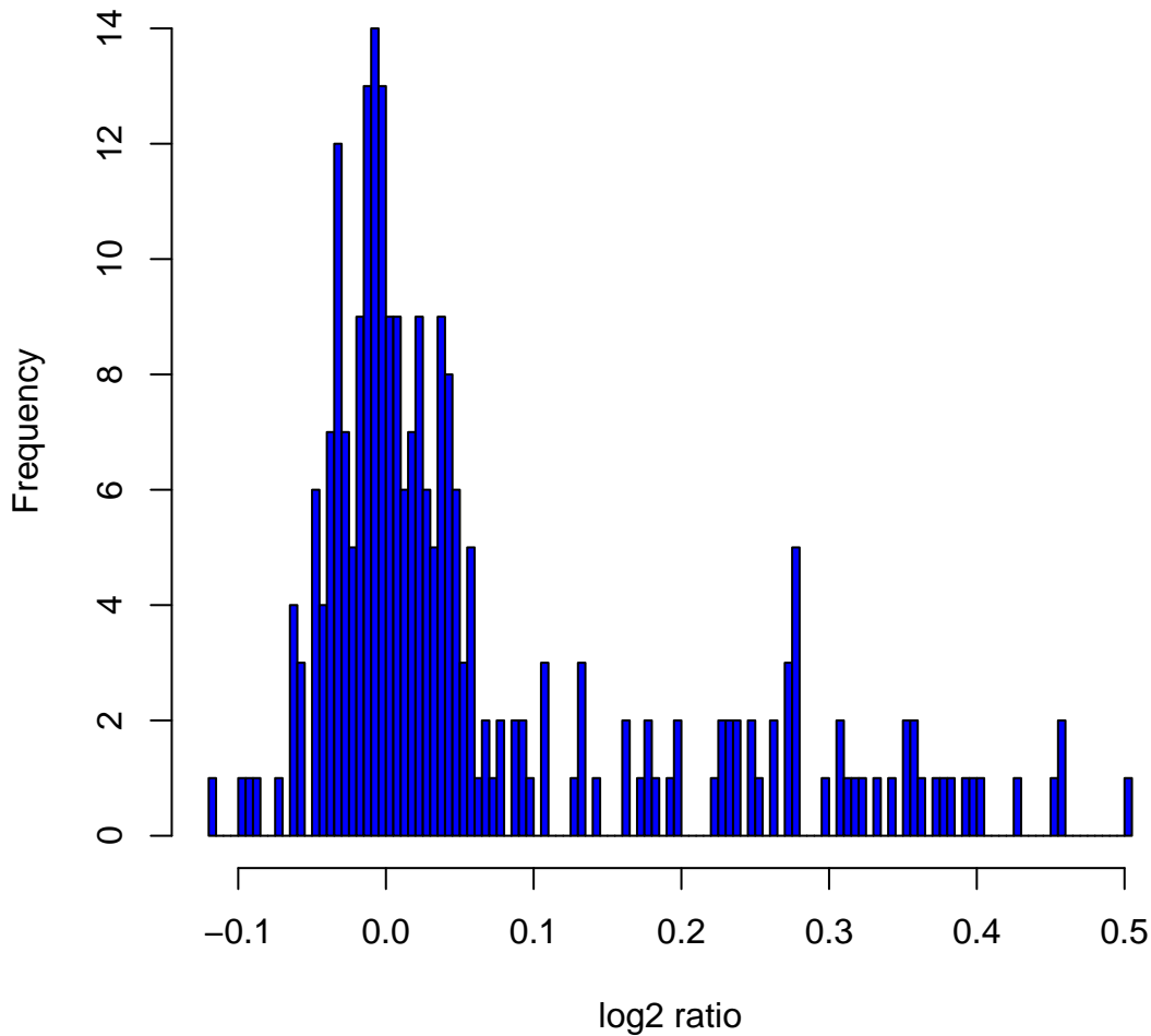
Histogram of log 2 ratios in 270 HapMap samples at clone Chr17tp-3D7
