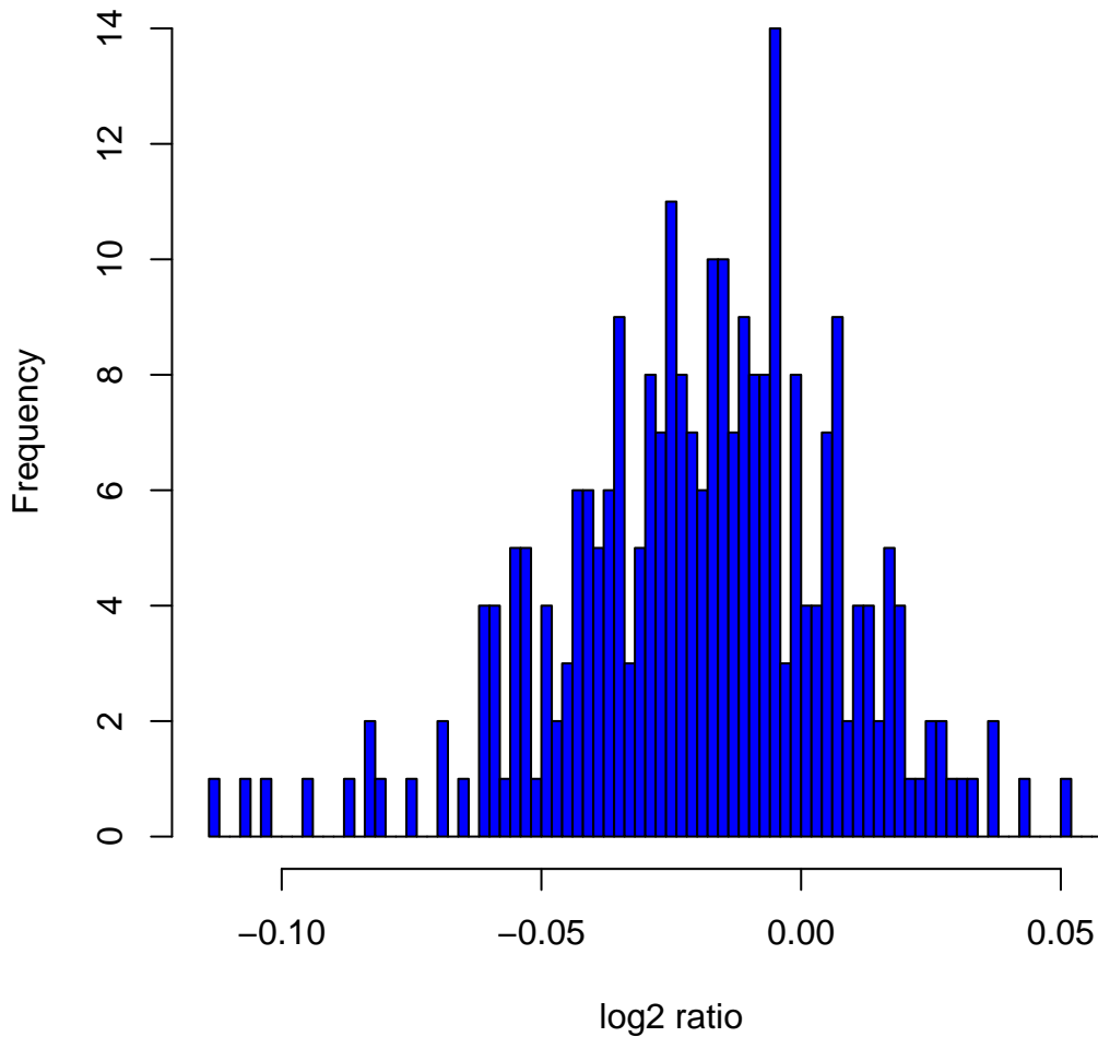
Histogram of log 2 ratios in 270 HapMap samples at clone Chr17tp-3E3
