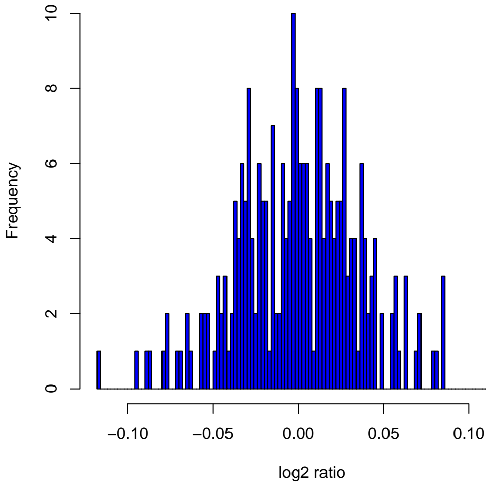
Histogram of \log_2 ratios in 270 HapMap samples at clone Chr17tp-3E5
