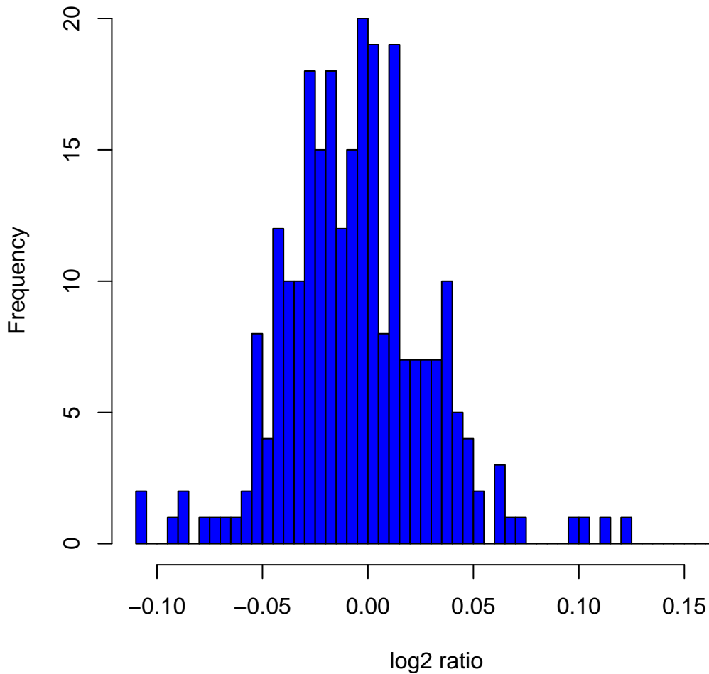
Histogram of log2ratios in 270 HapMap samples at clone Chr17tp-3G10
