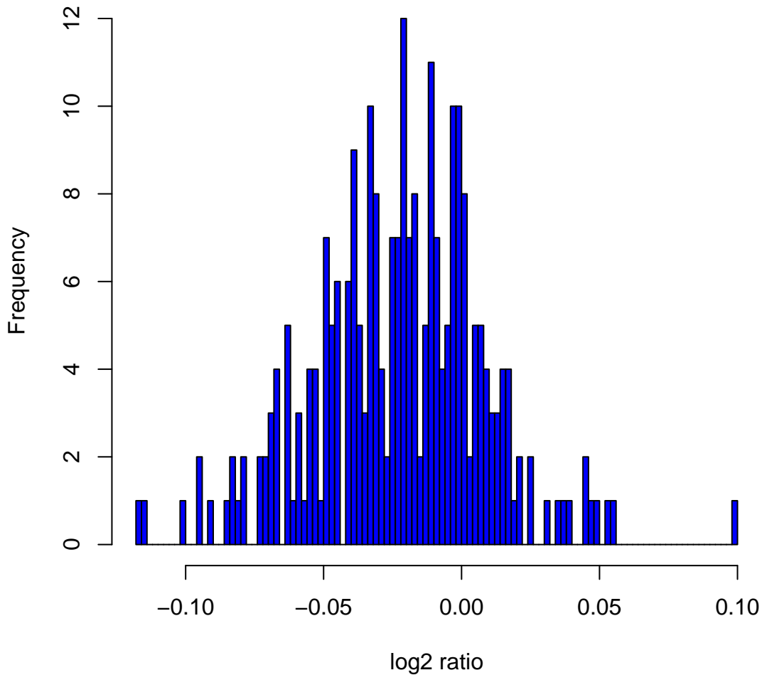
Histogram of \log_2 ratios in 270 HapMap samples at clone Chr17tp-3G4
