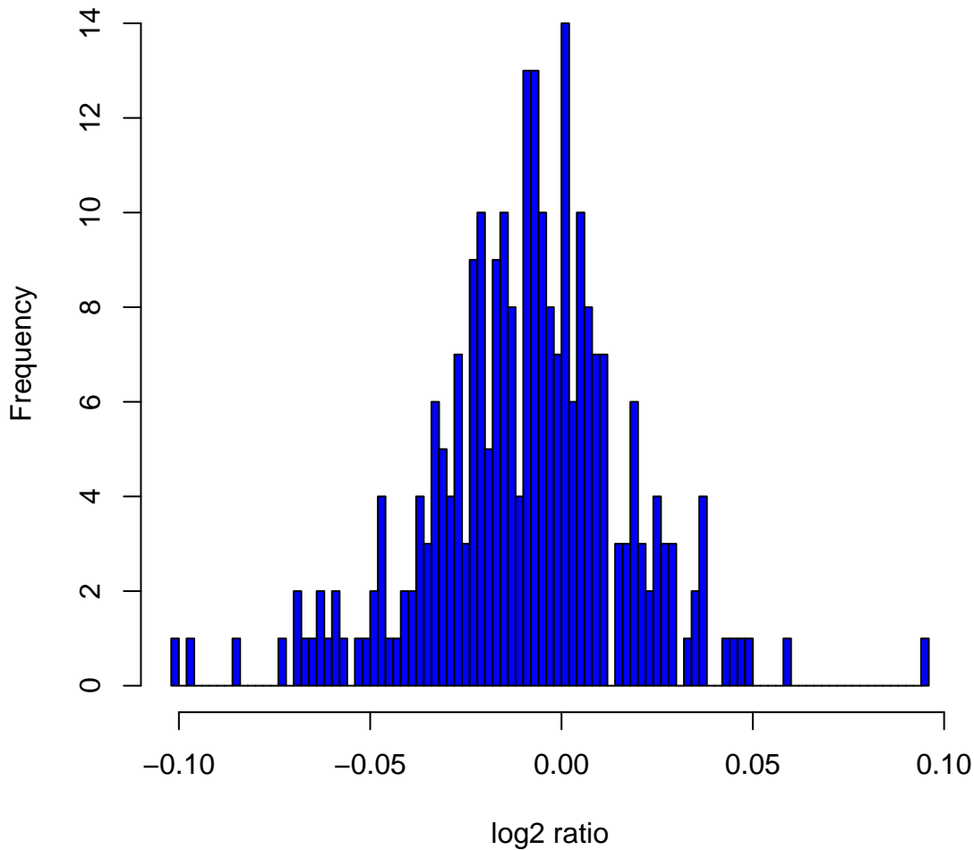
Histogram of log2ratios in 270 HapMap samples at clone Chr17tp-4A12
