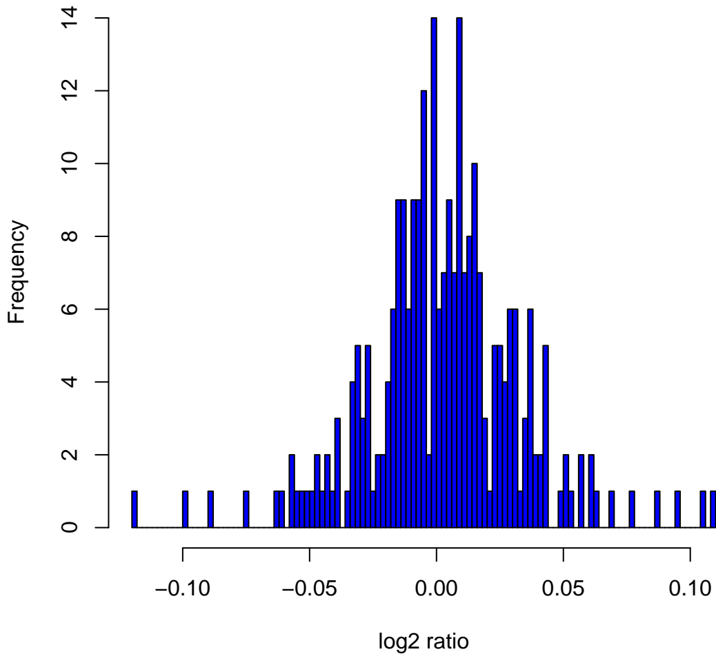
Histogram of log 2 ratios in 270 HapMap samples at clone Chr17tp-4A9
