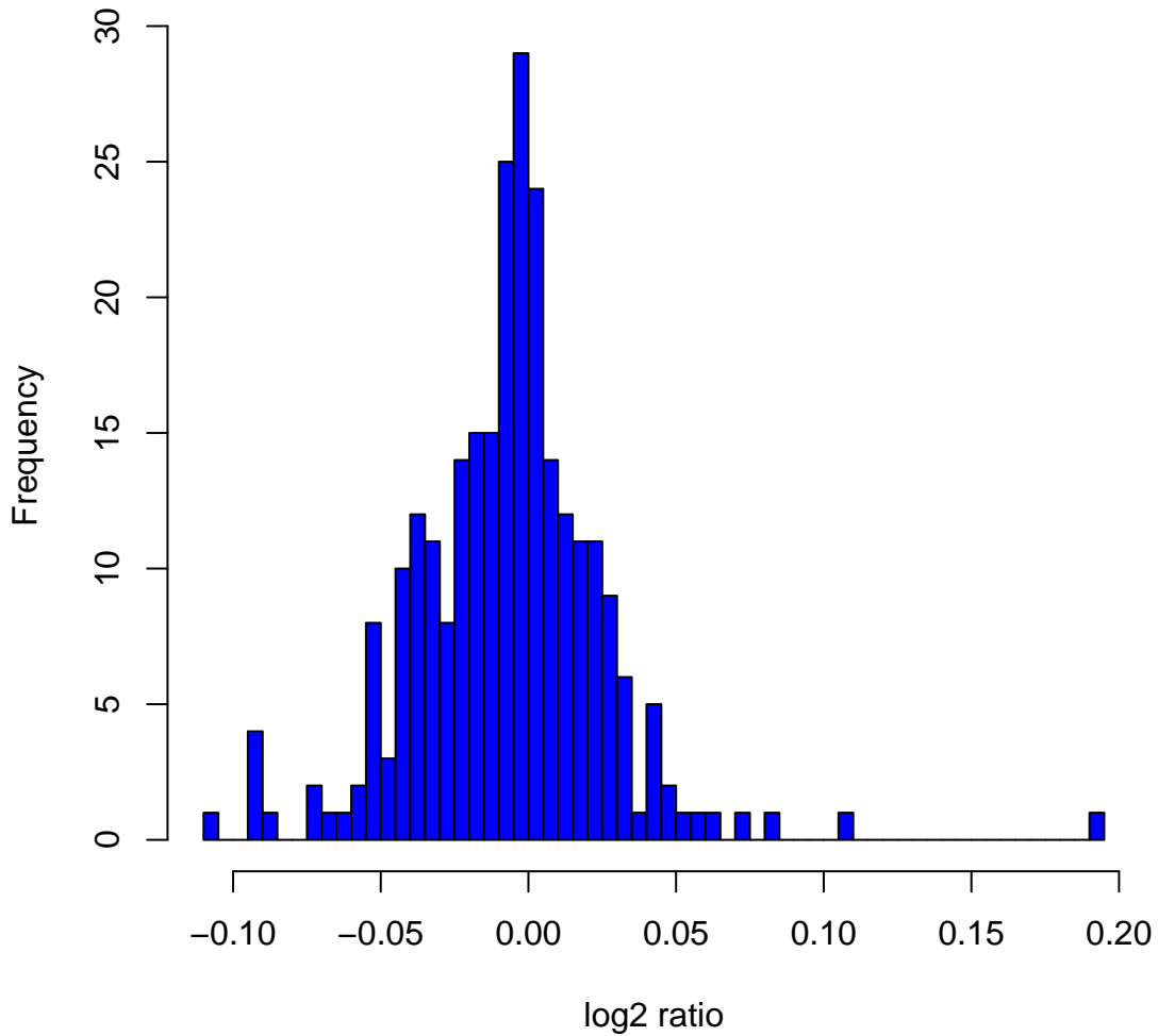
Histogram of log 2 ratios in 270 HapMap samples at clone Chr17tp-4B3
