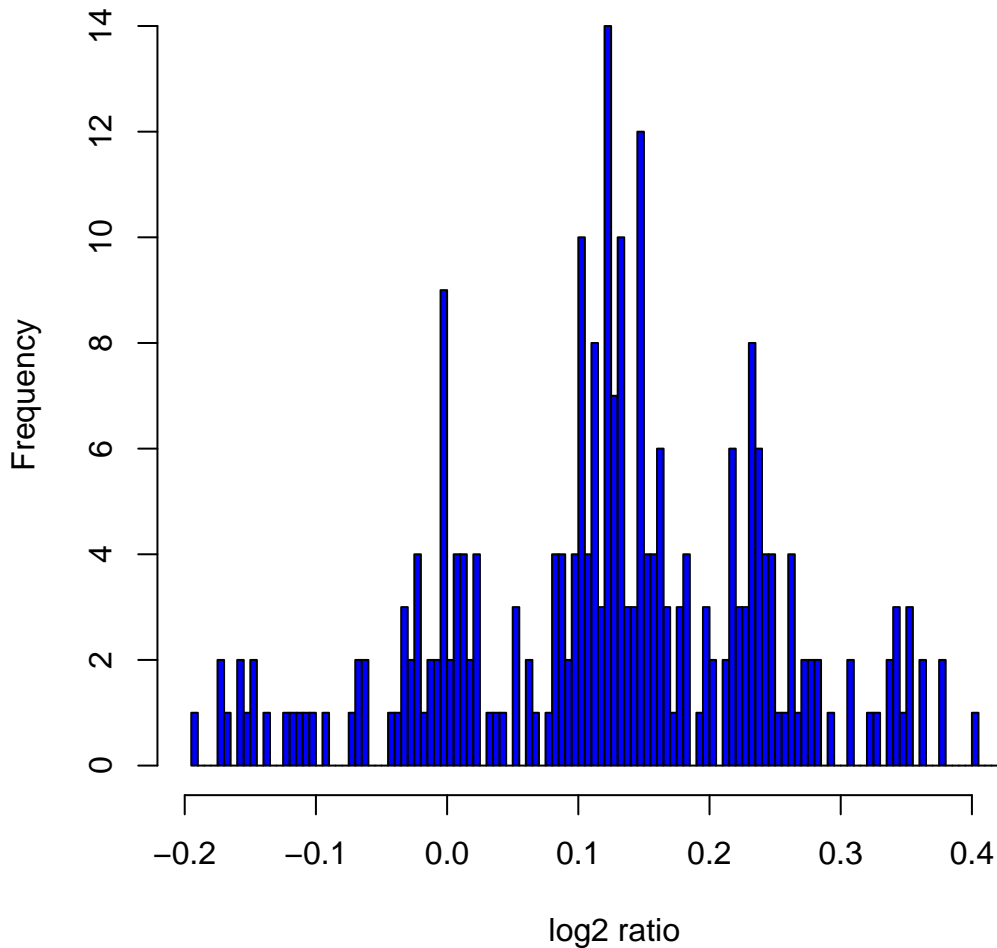
Histogram of log 2 ratios in 270 HapMap samples at clone Chr17tp-5A6
