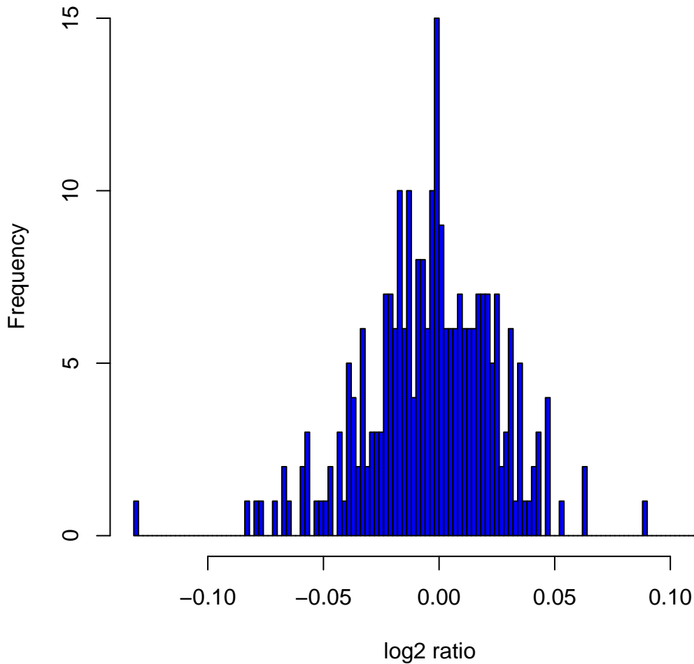
Histogram of log 2 ratios in 270 HapMap samples at clone Chr17tp-5B5
