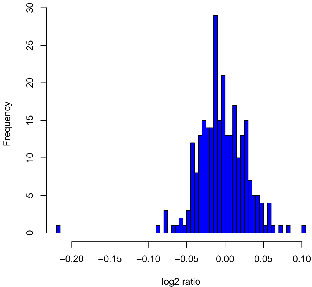
Histogram of log2ratios in 270 HapMap samples at clone Chr17tp-6A11
