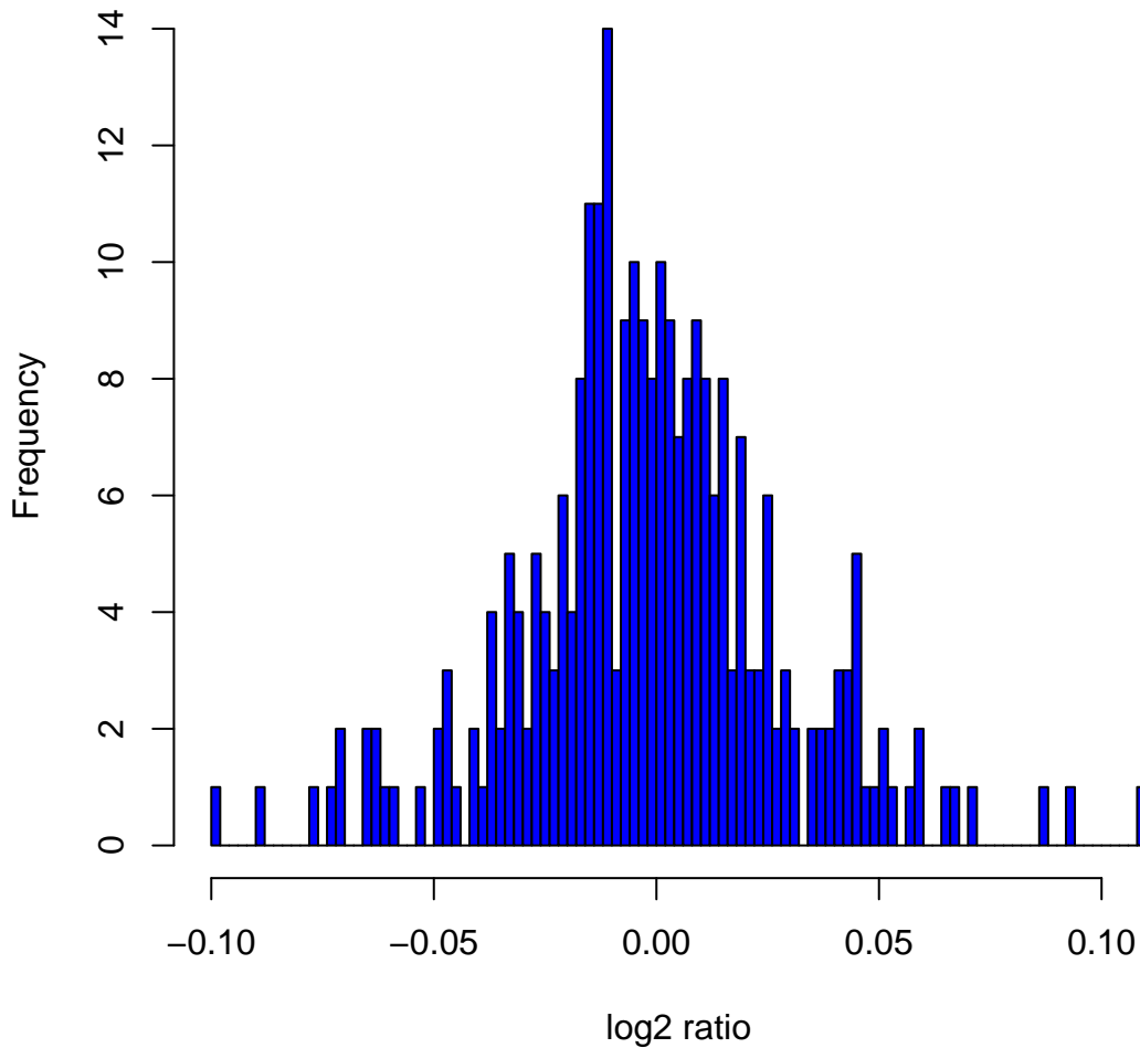
Histogram of \log_2 ratios in 270 HapMap samples at clone Chr17tp-6G4
