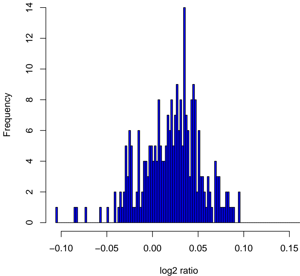
Histogram of \log_2 ratios in 270 HapMap samples at clone Chr17tp-6G6
