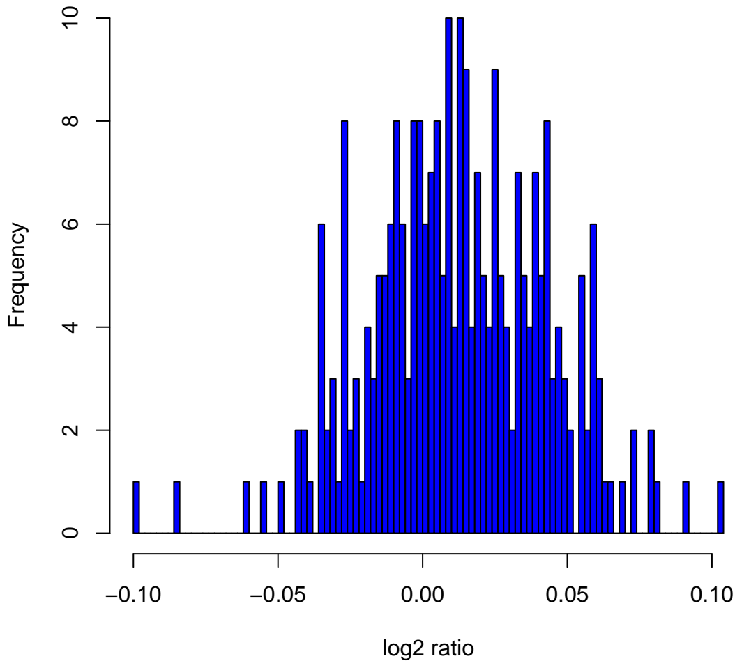
Histogram of \log_2 ratios in 270 HapMap samples at clone Chr17tp-6G7
