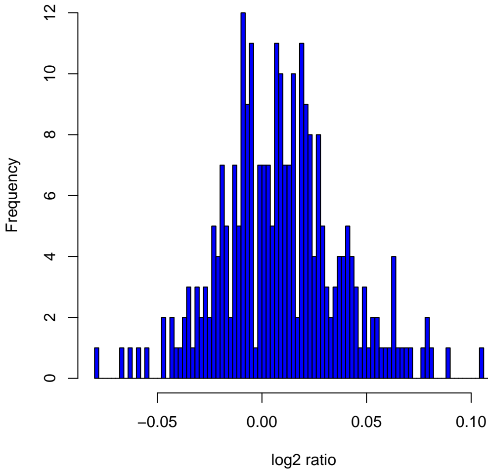
Histogram of log2ratios in 270 HapMap samples at clone Chr17tp-7A10
