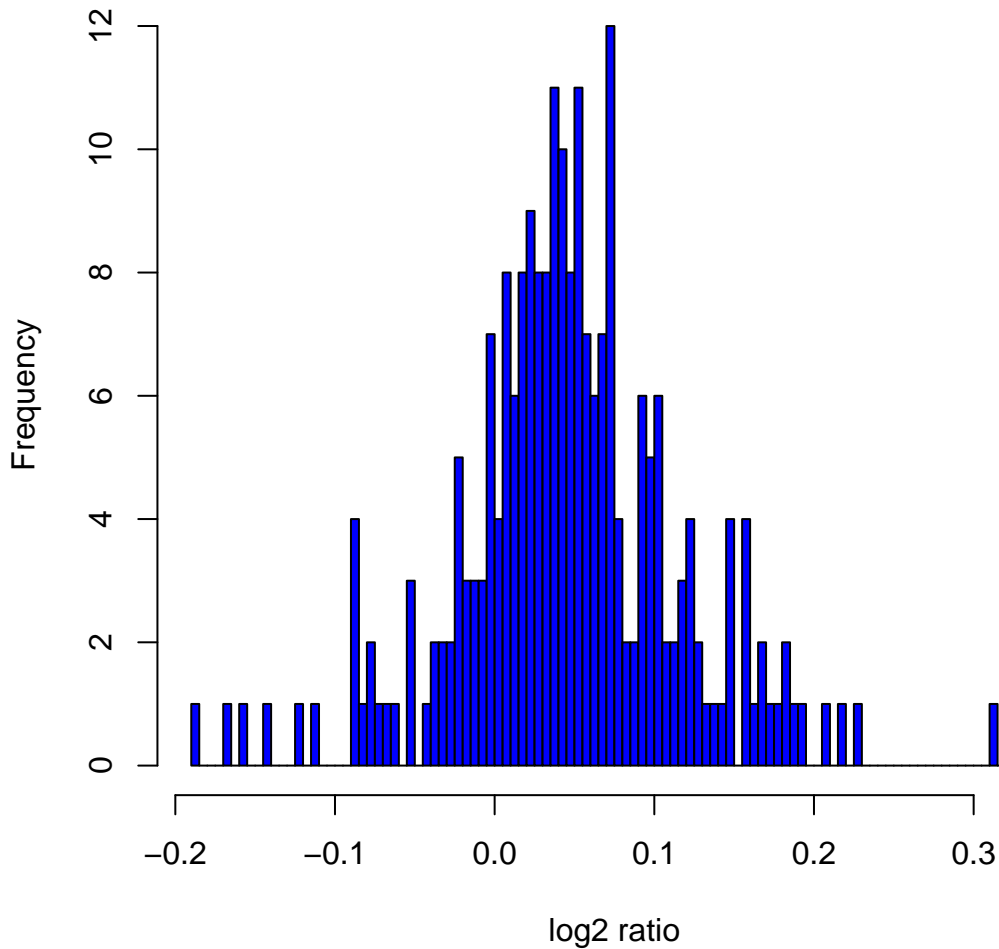
Histogram of log2ratios in 270 HapMap samples at clone Chr17tp-7B4
