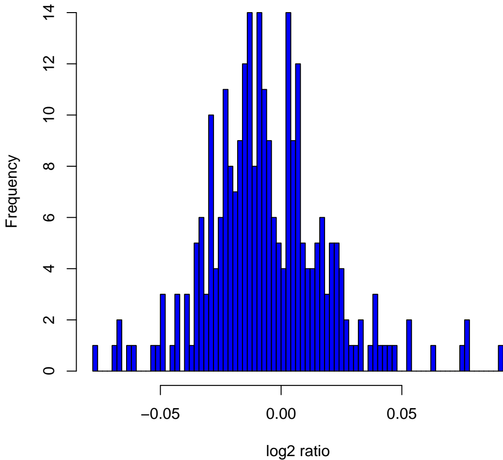
Histogram of log 2 ratios in 270 HapMap samples at clone Chr17tp-8B4
