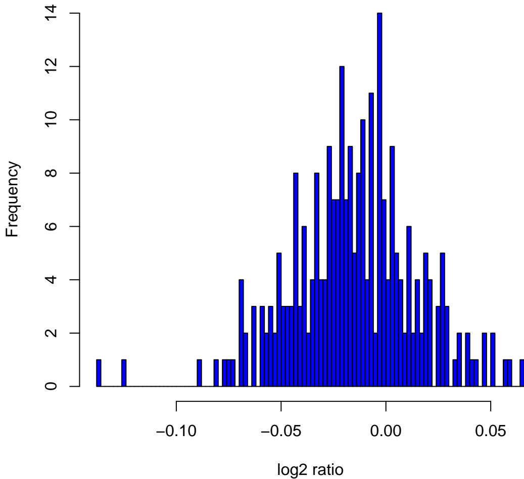
Histogram of log2ratios in 270 HapMap samples at clone Chr8tp-1B11
