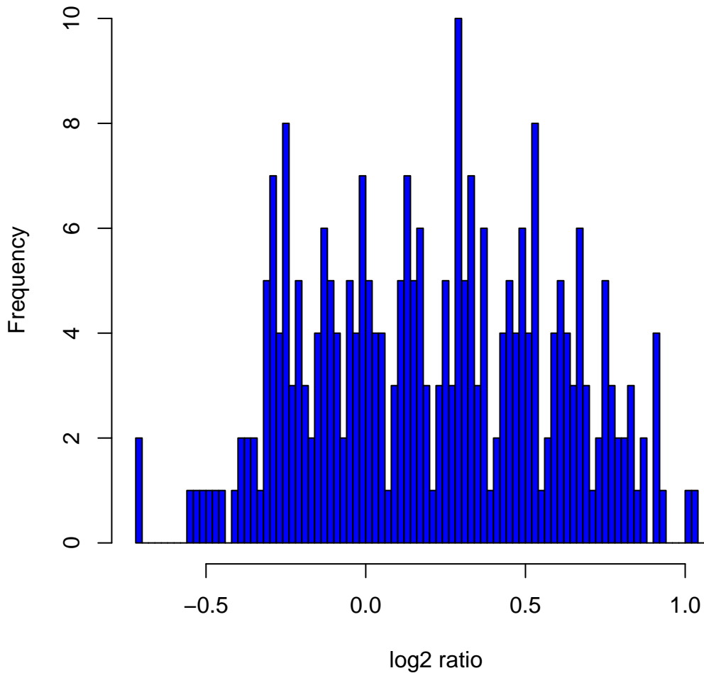
Histogram of log2ratios in 270 HapMap samples at clone Chr9tp-6G12
