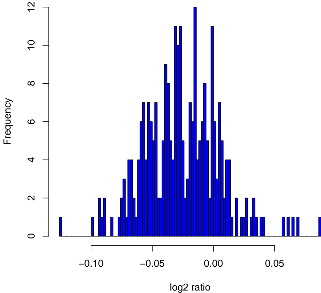
Histogram of log2ratios in 270 HapMap samples at clone Chr18tp-10A1
