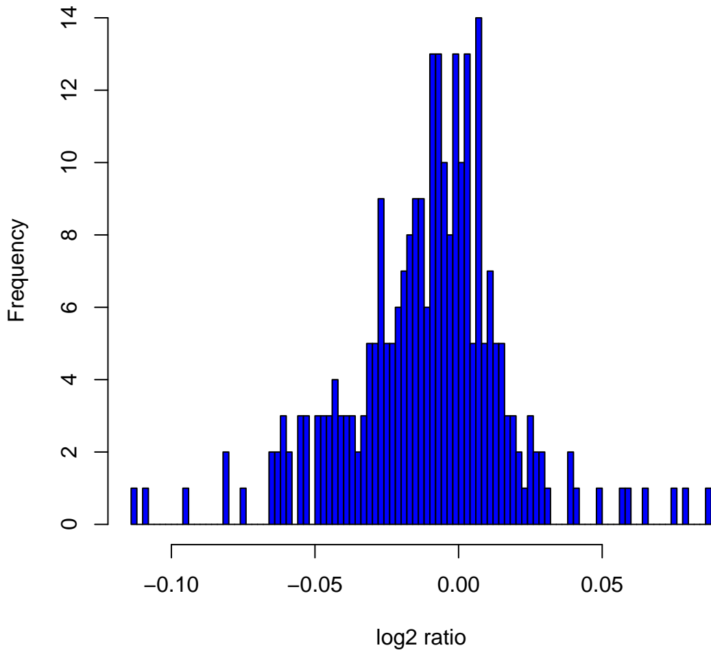
Histogram of log2ratios in 270 HapMap samples at clone Chr18tp-10B2
