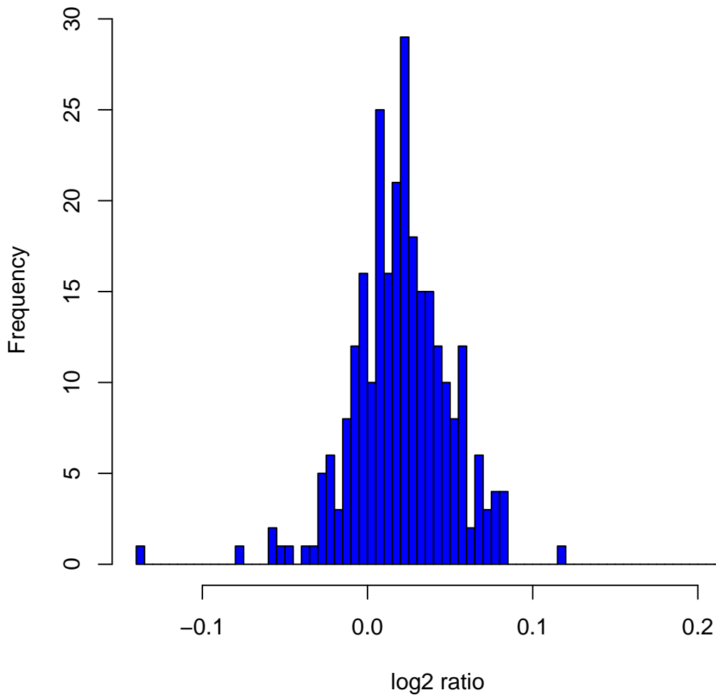
Histogram of \log_2 ratios in 270 HapMap samples at clone Chr18tp-10C4
