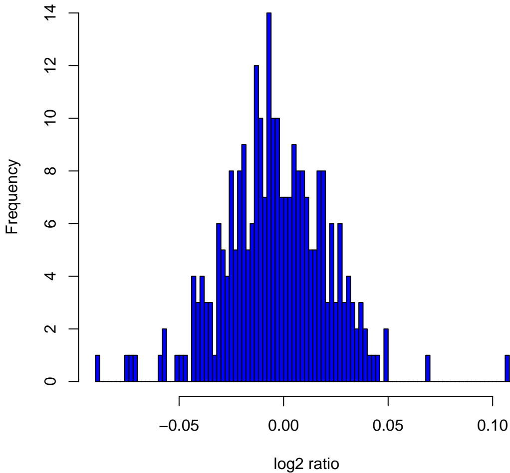
Histogram of log 2 ratios in 270 HapMap samples at clone Chr18tp-1A4
