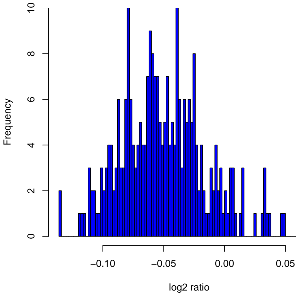
Histogram of log 2 ratios in 270 HapMap samples at clone Chr18tp-1G1
