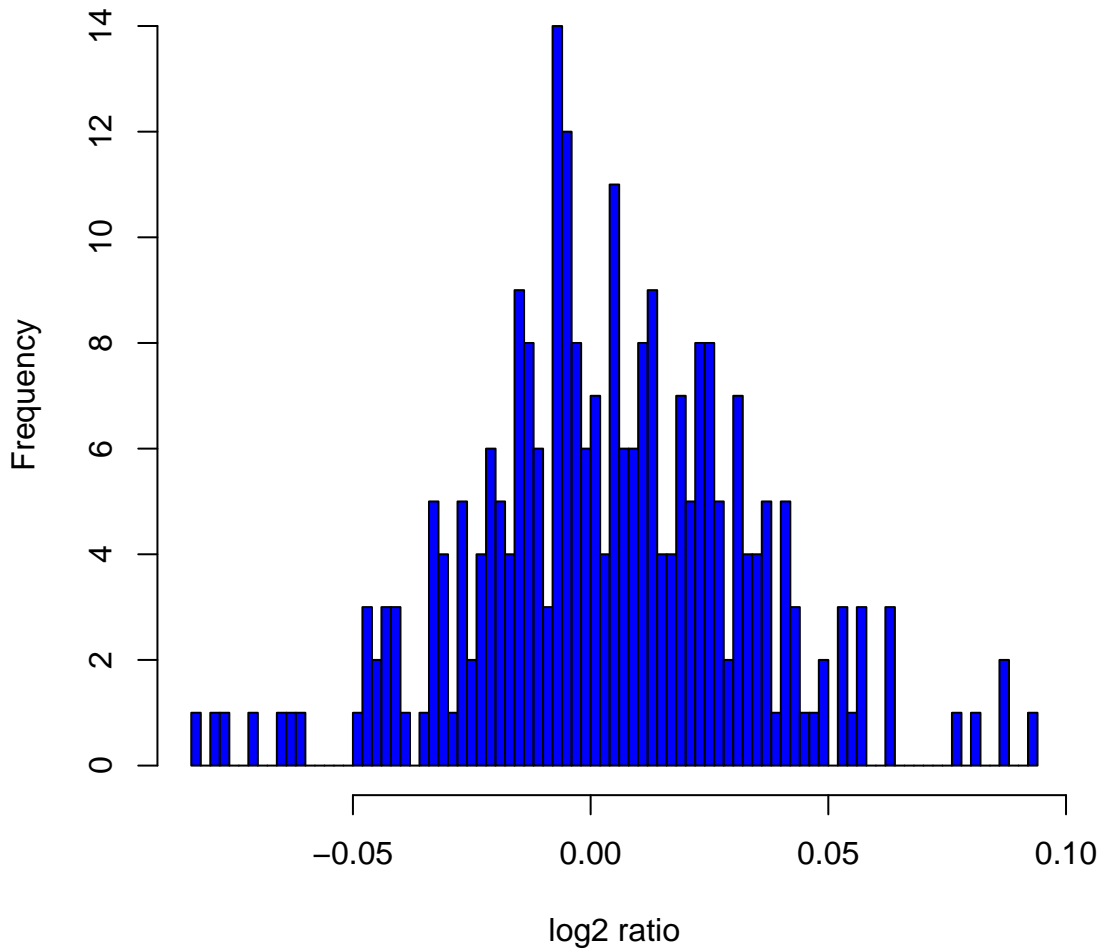
Histogram of log 2 ratios in 270 HapMap samples at clone Chr18tp-1G6
