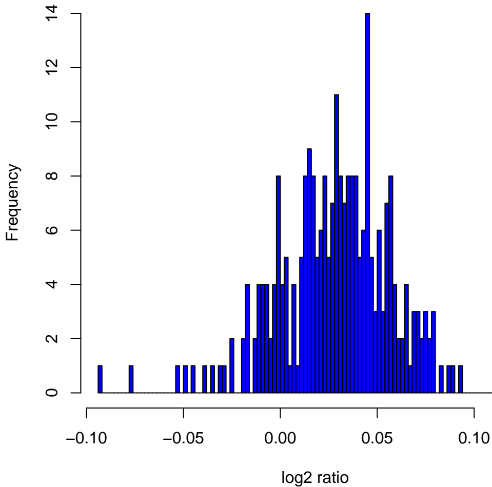
Histogram of log2ratios in 270 HapMap samples at clone Chr18tp-2B10
