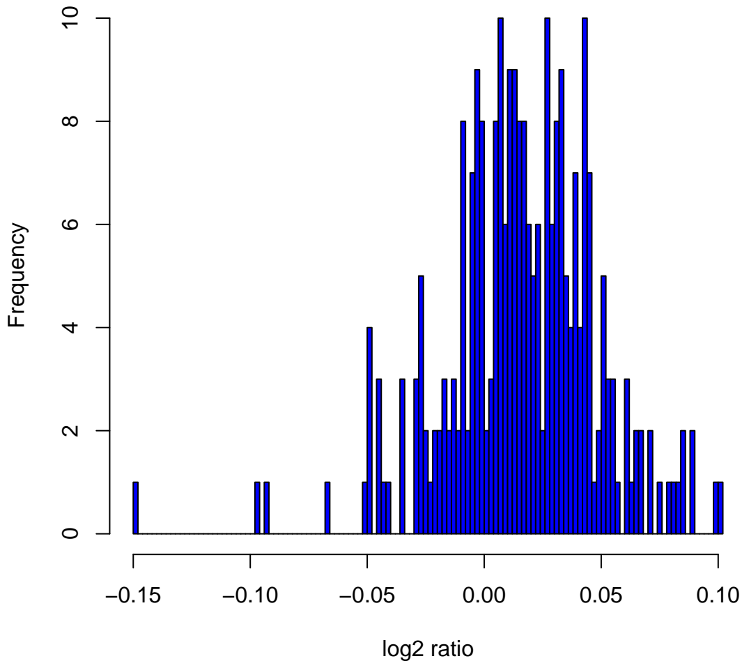
Histogram of log 2 ratios in 270 HapMap samples at clone Chr18tp-2D9
