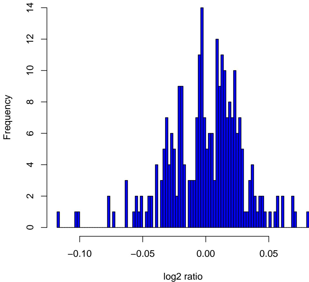
Histogram of log2ratios in 270 HapMap samples at clone Chr18tp-2E1
